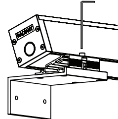
Turn Allen Key to adjust angle
