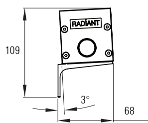
Fixed angle bracket
