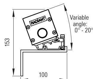
Adjustable angle bracket
